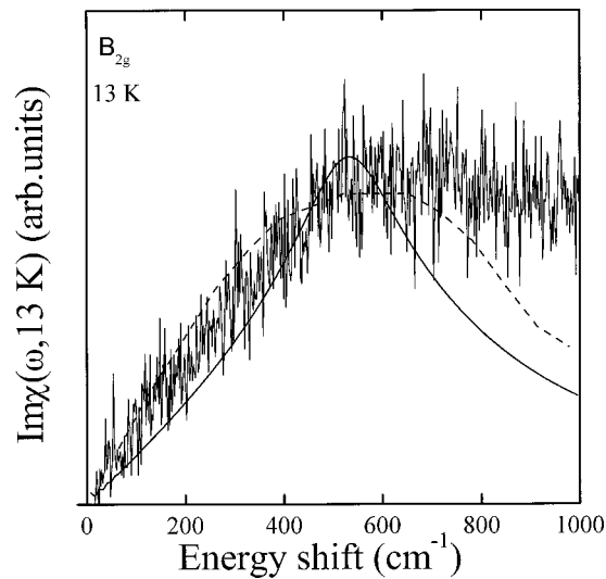
FIG. 10. B_{2g} data (sample A) and calculations for the d_{x^2-y^2} model (dashed line) and for a model with 8 nodes lying at \theta_0=26^\circ (solid line).
